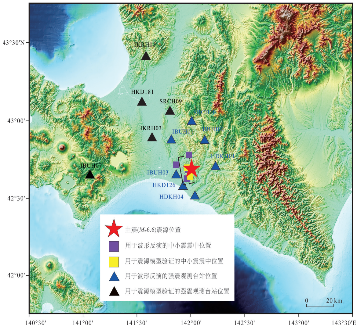
图 1 2018年日本北海道 M_w 6.6地震及波形反演中选取的中小震震中位置、发震断层和所选取的强震观测台站 Fig.1 Location of hypocenters of the 2018 Hokkaido earthquake and the small events used in the inversion analysis
