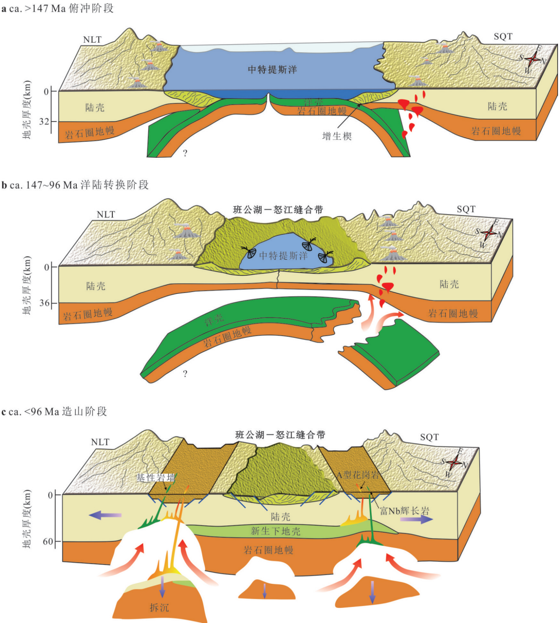
图 10 中晚侏罗世—白垩纪中特提斯洋洋陆转换与造山过程演化示意图 Fig. 10 Schematic diagram of ocean-continent transition and orogenic process evolution of the Meso-Tethys Ocean during the Middle-Late Jurassic - Cretaceous 缩写: SQT, 南羌塘地体, NLT, 北拉萨地体
