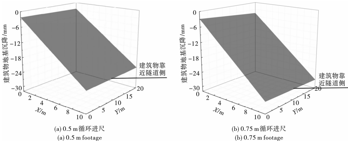
图9 不同工况下建筑物沉降 Fig. 9 Building settlement under different working conditions
