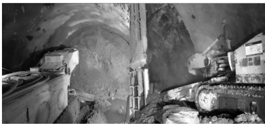
(a) 上断面机械法施工 (a) Mechanical construction of the upper bench
