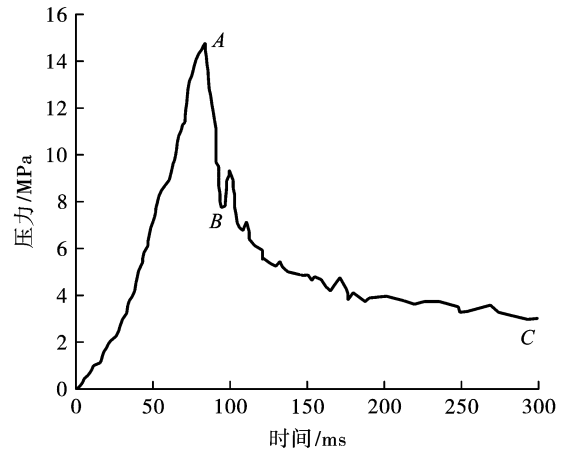
图 4 高压气体爆破冲击下致裂孔壁的压力时程曲线 Fig. 4 Pressure curve of cracking hole wall under high-pressure gas blasting
