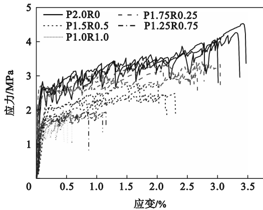
图6 RTP-PVA 混杂纤维ECC 应力-应变曲线 Fig. 6 Stress-strain curves of RTP-PVA hybrid fibre reinforced ECC
