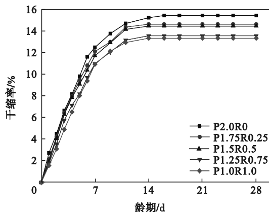
图7 RTP-PVA 混杂纤维ECC 干缩率 Fig. 7 Drying shrinkage rate of RTP-PVA hybrid fibre reinforced ECC
