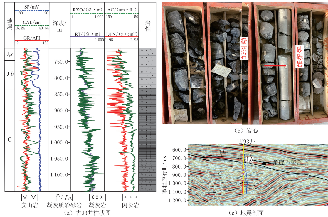
图 6 克百断裂带古 93 井火山旋回划分标志 Fig. 6 Division of volcanic cycles in the well Gu 93 of the Kebai Fault Zone
