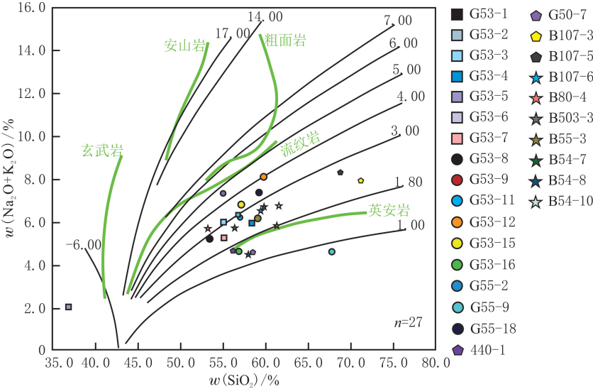
图 4 克百断裂带上盘石炭系火山岩里特曼指数 Fig. 4 Rittmann index of the Carboniferous volcanic rocks on the hanging wall of the Kebai Fault Zone
