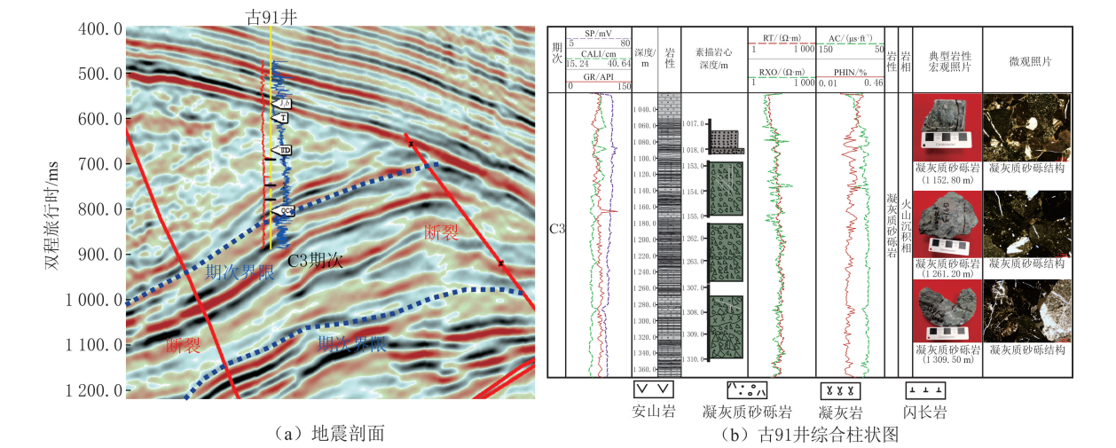
图 9 克百断裂带上盘石炭系 C3 期次划分 Fig. 9 Division of C3 sequences of the Carboniferous volcanic rocks on the hanging wall of the Kebai Fault Zone
