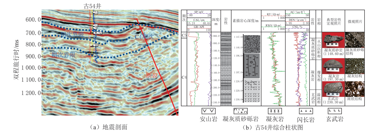
图 10 克百断裂带上盘石炭系 C4 期次 Fig. 10 Division of C4 sequences of the Carboniferous volcanic rocks on the hanging wall of the Kebai Fault Zone
