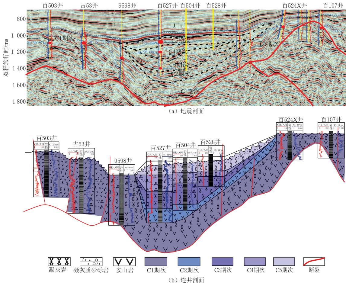
Fig. 12 The crosssection wells of the Carboniferous volcanic rocks on the hanging wall of the Kebai Fault Zone
