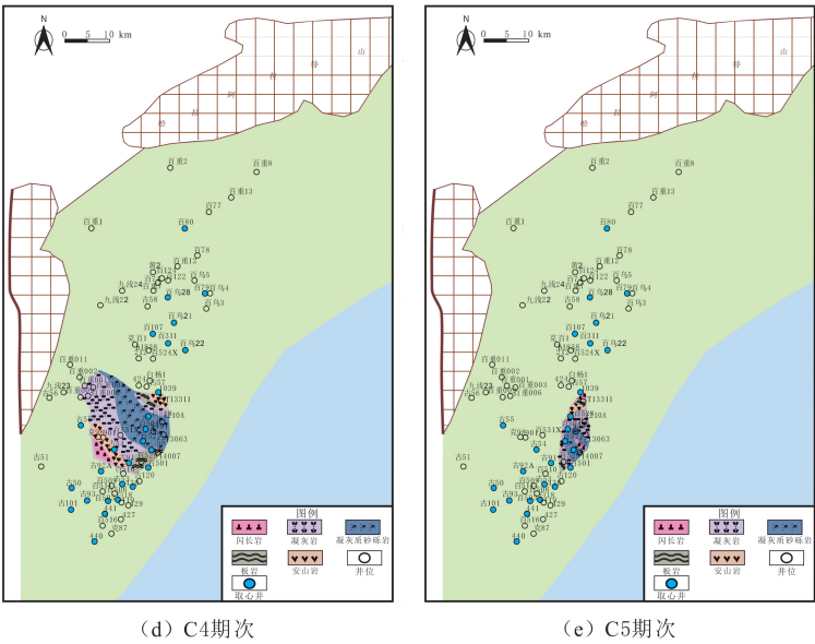
图 13 克百断裂带上盘石炭系期次与火山岩岩性平面分布 Fig. 13 Distribution pattern of the Carboniferous volcanic rocks on the hanging wall of the Kebai Fault Zone
