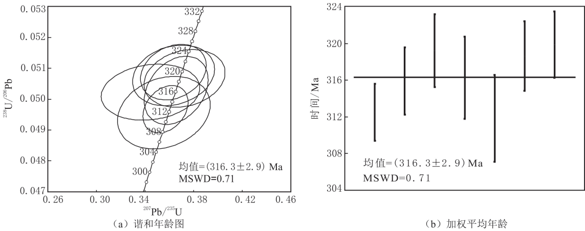
图 5 克百断裂带百 527 井凝灰岩锆石 U-Pb 同位素年龄谐和图与年龄谱图 Fig. 5 Zircon U-Pb concordial diagram and age histogram of tuff zircons from well Bai 527 of Kebai Fault Zone
