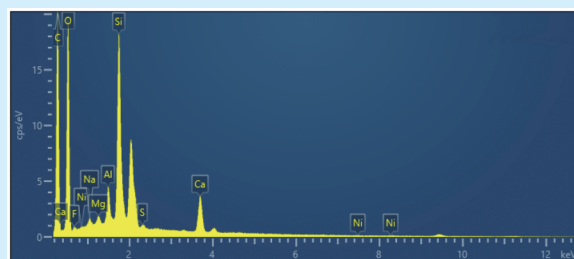
The contents of main elements on dentin surface were C (52.02 wt%), O (38.35 wt%), and Si (5.02 wt%). EDX: energy dispersive X-ray spectroscopy
