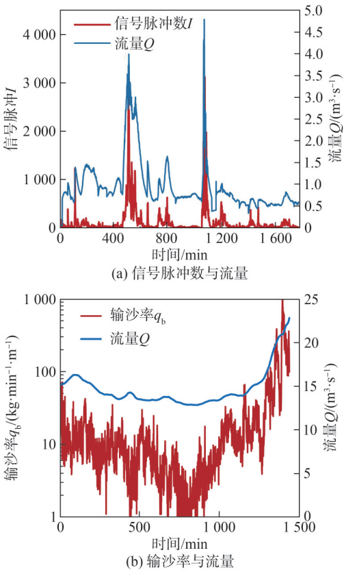
图10 瑞士Erlenbach及Fischbach山区河流推移质信号脉冲及输沙率与流量的关系 [49,81] Fig. 10 Relationships of bedload-generated signal impulses, bedload transport rate, and flow discharge in the Swiss mountain streams Erlenbach and Fischbach [49,81]
