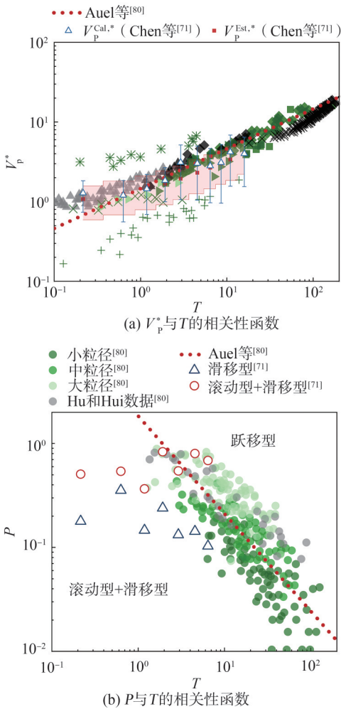
图9 无量纲推移质输移速度 V_p^* 、输移模式概率 P 与无量纲水力强度 T 的相关性 [71] Fig. 9 Nondimensional particle velocity V_p^* and probability of transport mode P as functions of the excess transport stage T [71]
